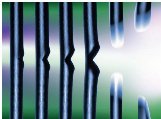
Fig.1: Crack propagation in a filament of polystyrene melt in extension flow, captured by the high-speed camera.
